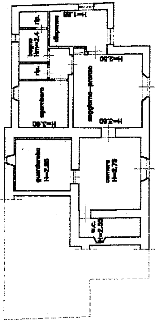
PIANO TERRA
